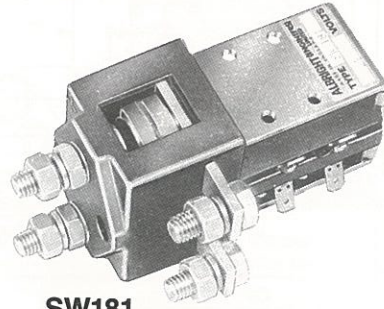
SW181 Single pole changeover contactor
