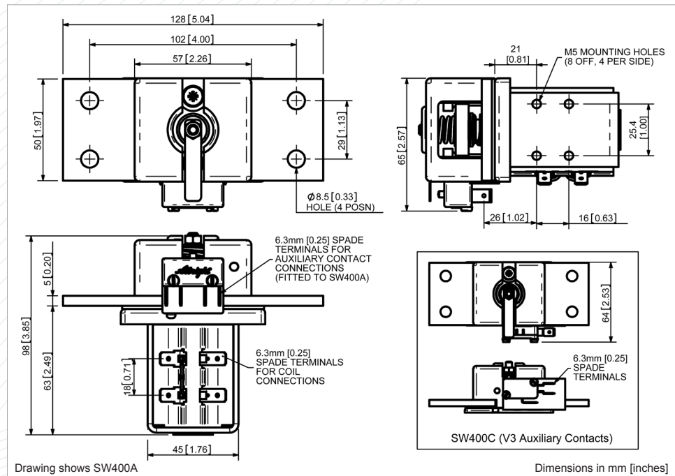
Drawing shows SW400A
